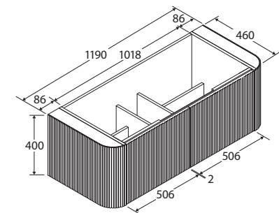
TOP VIEW: DRAWER AREA
