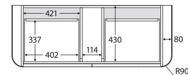
SIDE VIEW: DRAWER STORAGE
