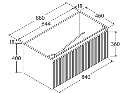
TOP VIEW: DRAWER AREA
